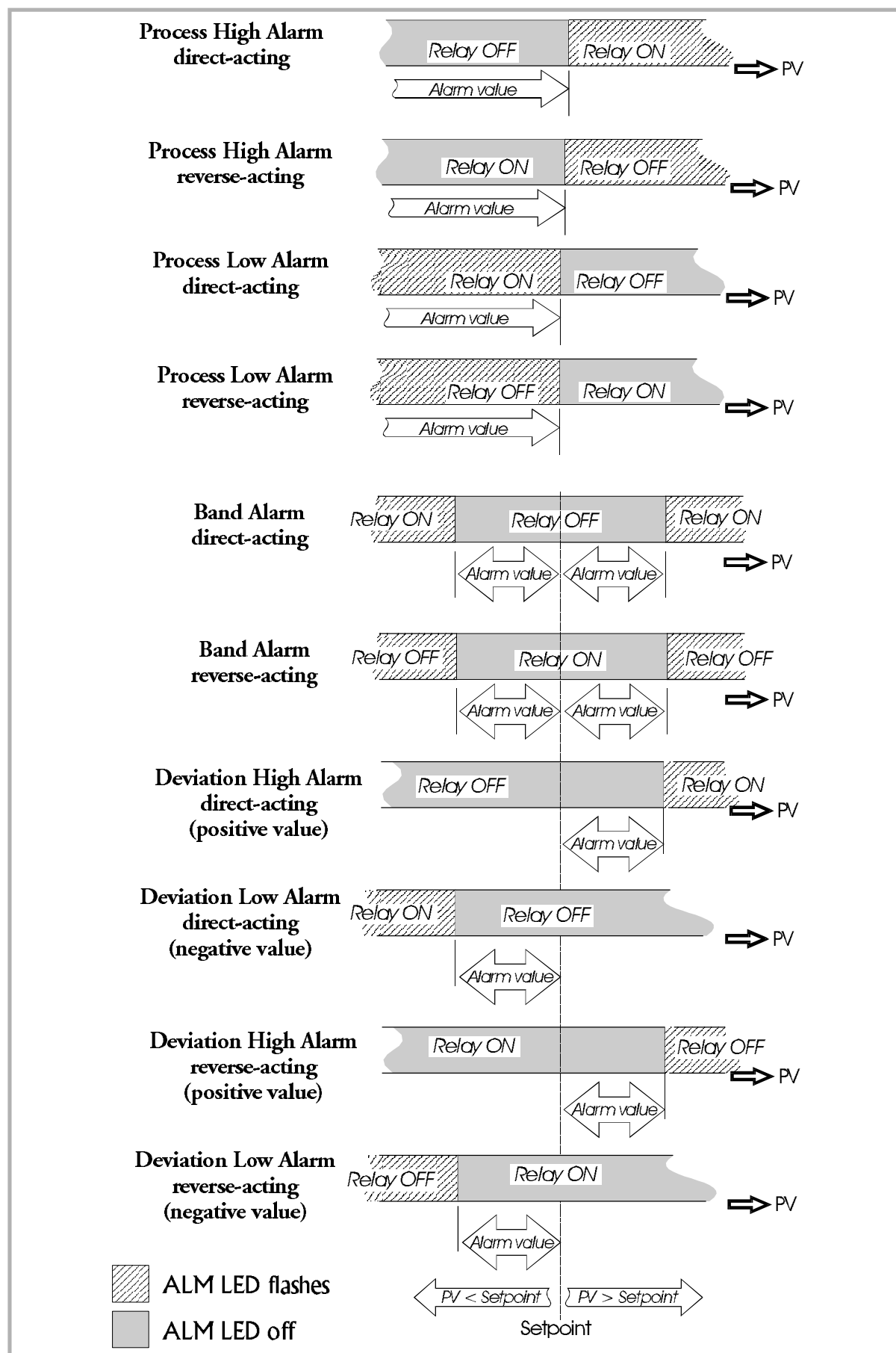
Figure 3-2 Alarm Operation
