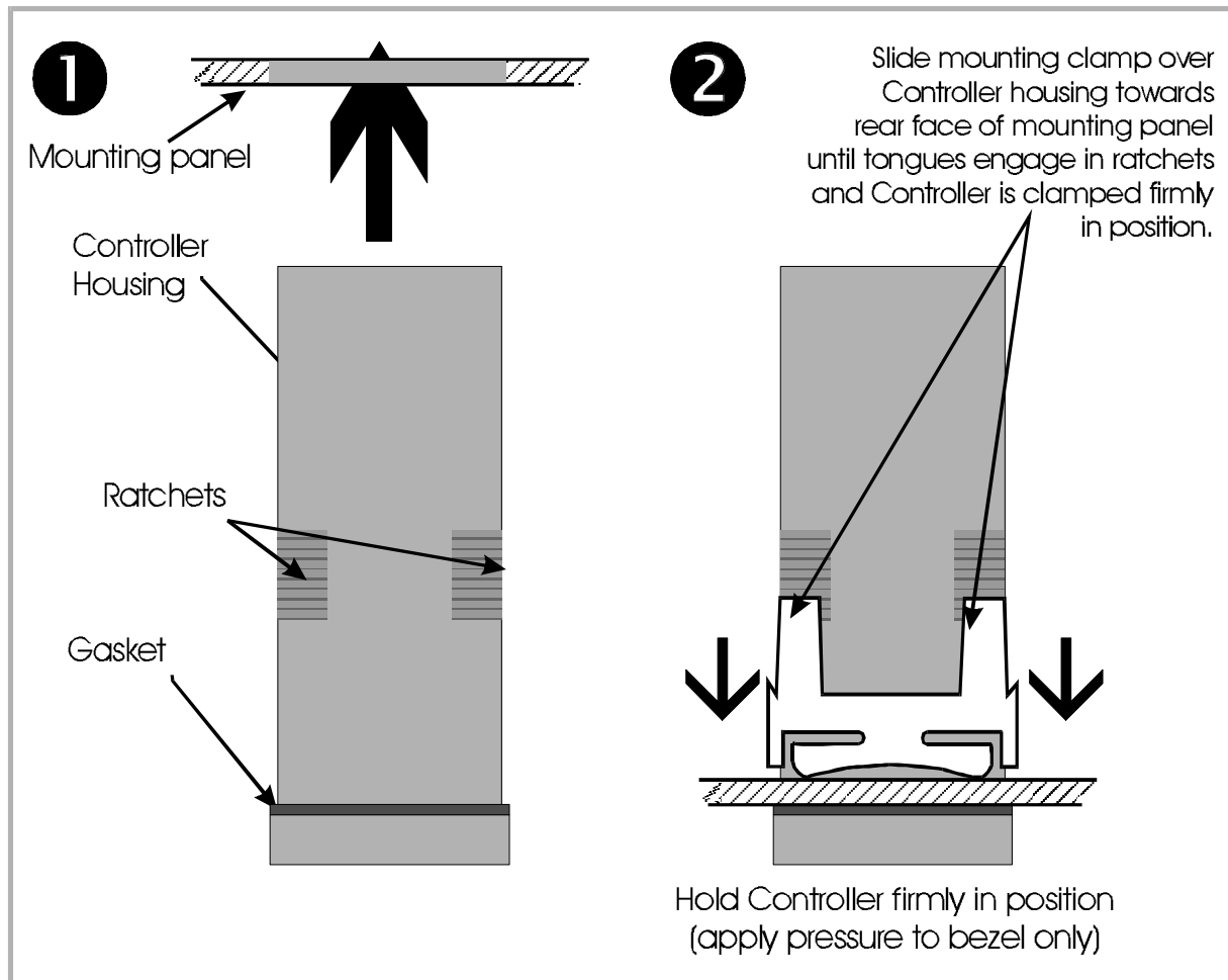
Figure 1-3 Panel-Mounting the Profiler/Controller
