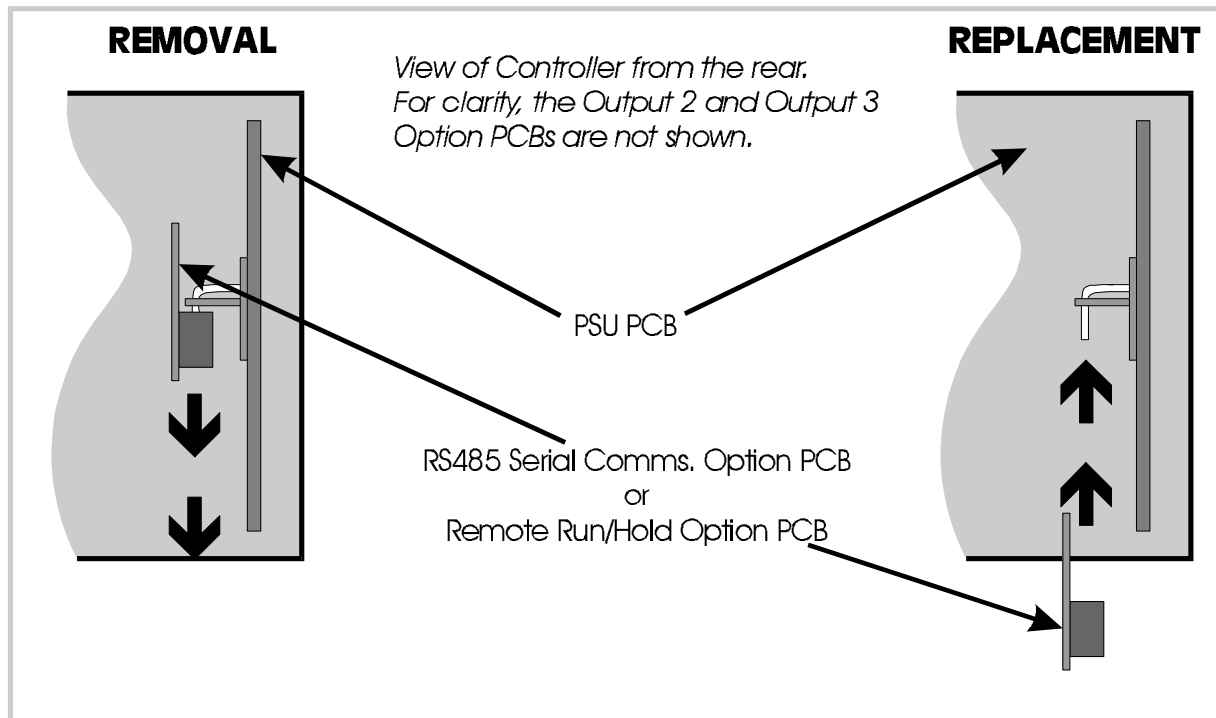
Figure 2-3 Removing the RS485 Communications Option PCB or the Remote Run/Hold Option PCB
