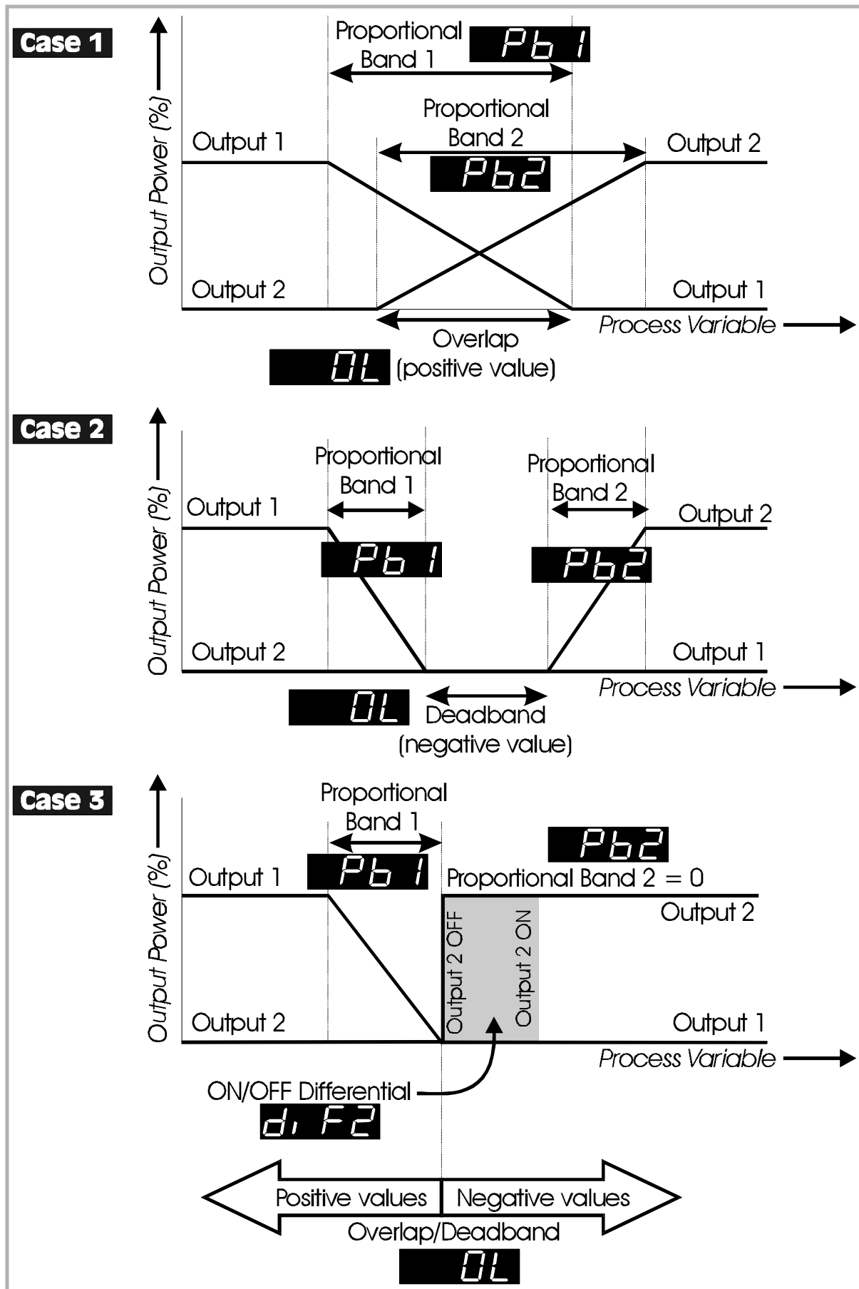
Figure 3-1 Proportional Band and Overlap/Deadband
