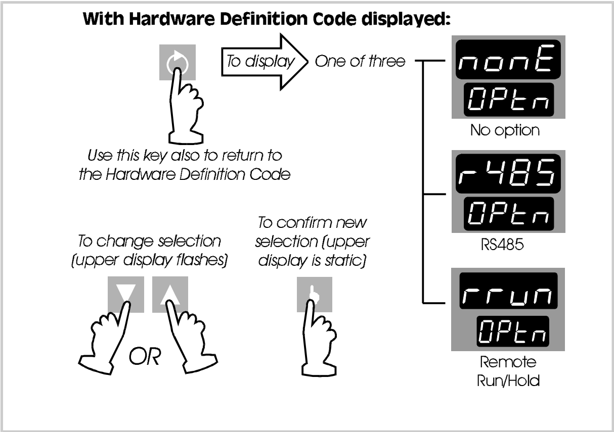
Figure 3-3 Option Selection
