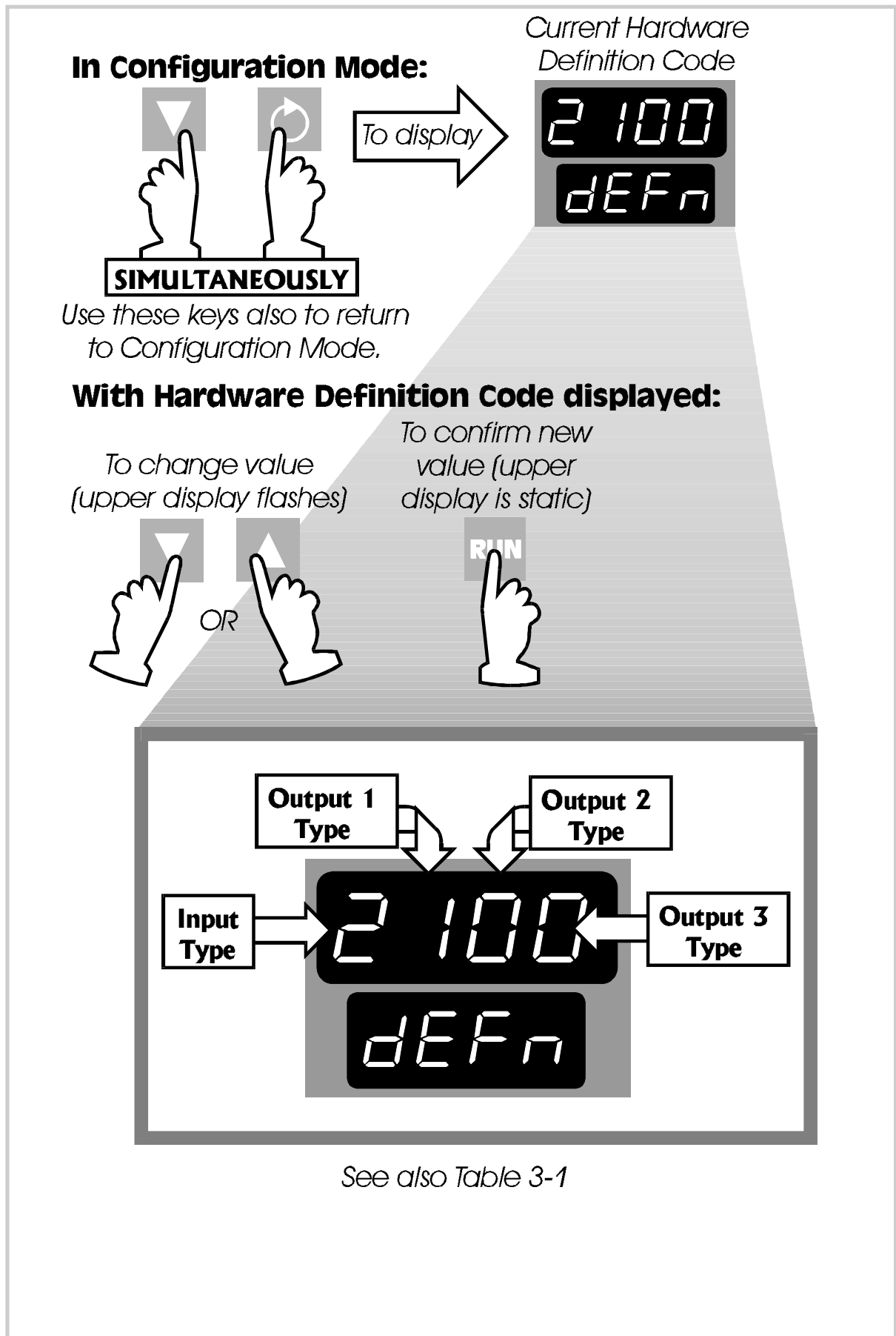
Figure 3-2 Hardware Definition Code - Access and Adjustment
