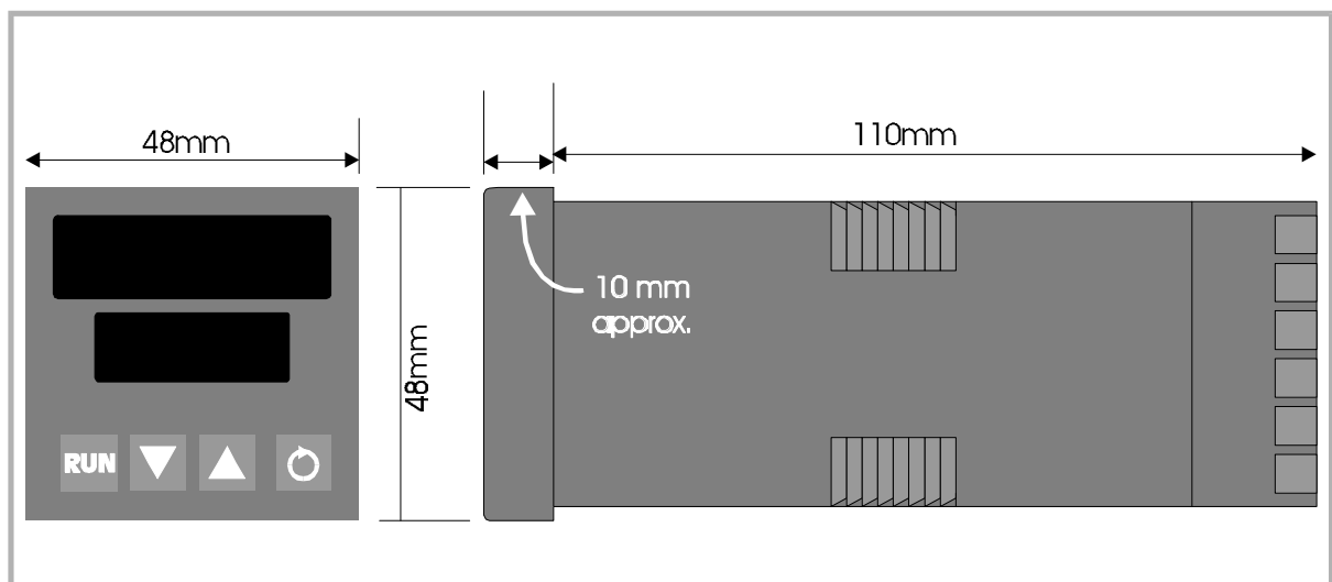
Figure 1-2 Main Dimensions
