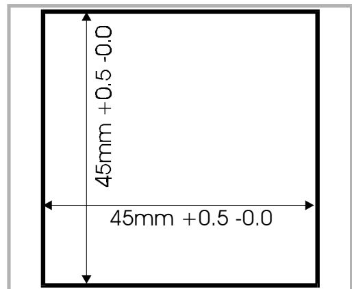
Figure 1-1 Cut-out Dimensions
