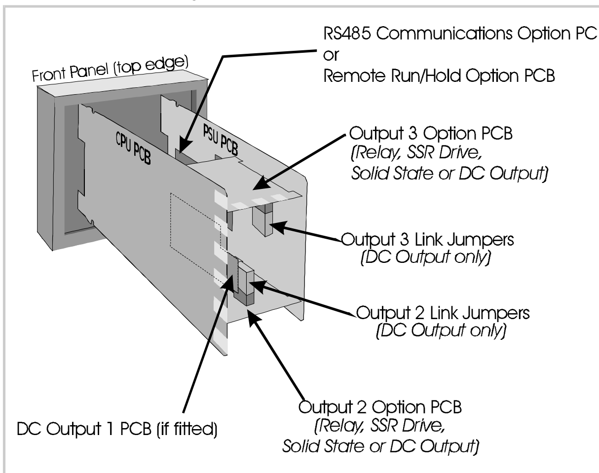
Figure 2-1 PCB Positions
