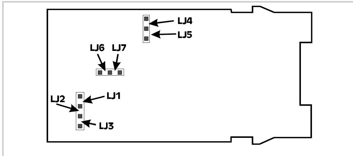
Figure 2-4 CPU PCB (Relay/SSR Drive/Solid State Output 1)
